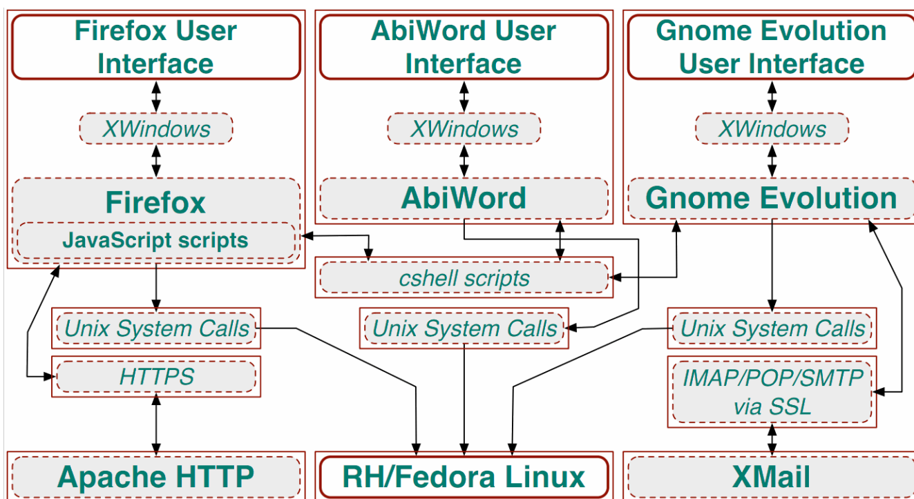
Secure build-time architecture for generic software applications available for use in C2 systems, from Scacchi and Alspaugh [2011].
