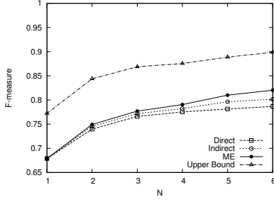
Fig. 15. F-measure vs. N .
