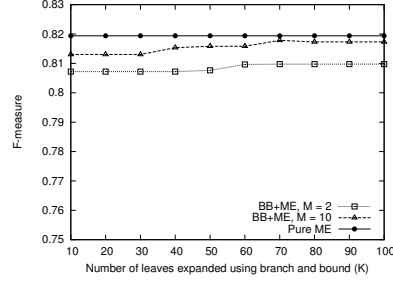
Fig. 17. Quality of BB Algorithm.
