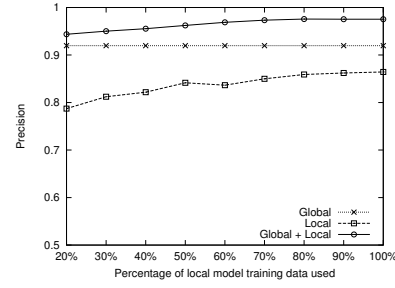
Fig. 21. Multimodel Test: Precision.
