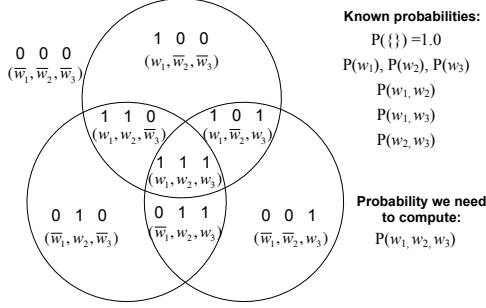
Fig. 2. Probability Space.
