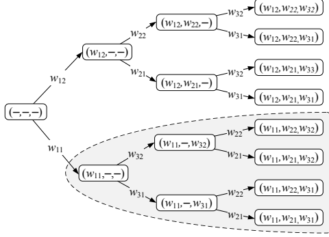
Fig. 7. Search Tree.
