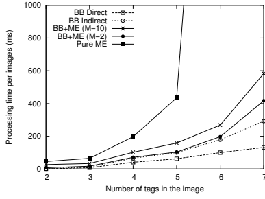
Fig. 19. Processing time.
