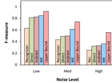
Fig. 14. F-measure vs. Noise.
