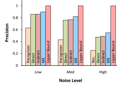
Fig. 12. Precision vs. Noise.
