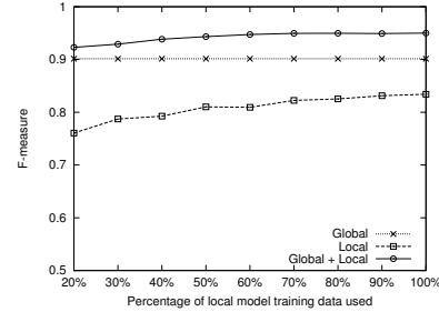
Fig. 23. Multimodel Test: F-Measure.
