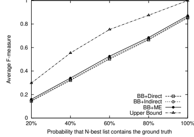
Fig. 18. Quality on a Larger Dataset.
