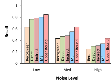
Fig. 13. Recall vs. Noise.
