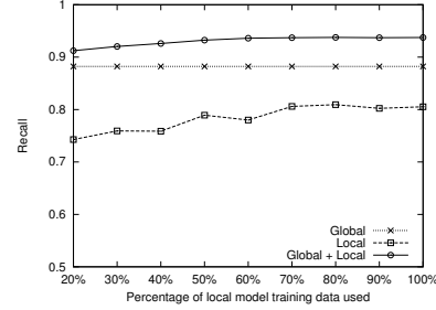
Fig. 22. Multimodel Test: Recall.
