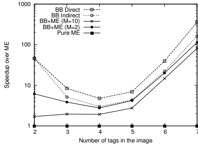
Fig. 20. Speedup of BB Algorithm.
