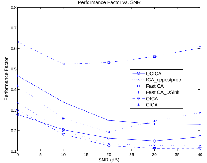
(b) Mean performance factor vs. SNR
