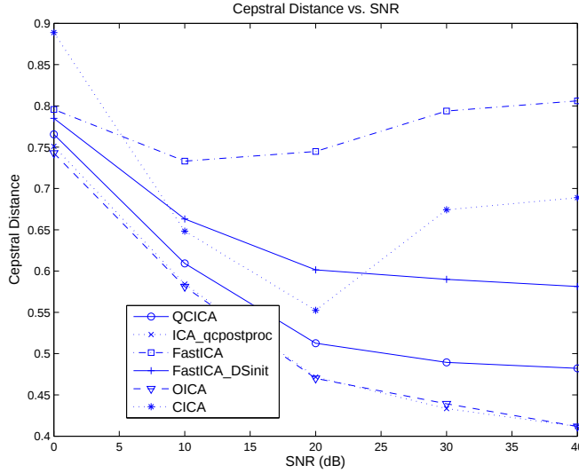
(a) Cepstral distance vs. SNR
