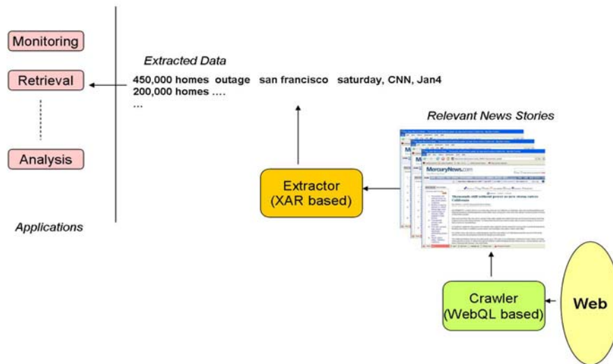
Fig 5. Internet Information Monitoring
