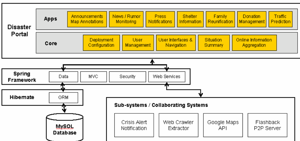
Fig 2. Disaster Portal System Architecture
