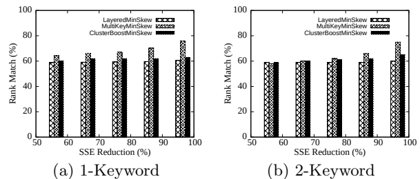
Figure 2: Rank Evaluation.
