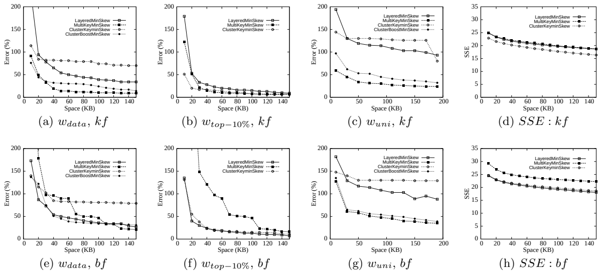
Figure 1: Results.
