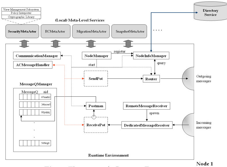
Fig. 3. The CompOSE|Q Runtime Environment
