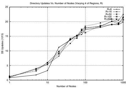
Fig. 6. Directory update overhead with varying number of nodes.
