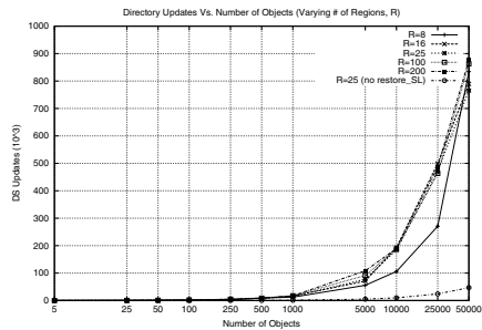
Fig. 5. Directory update overhead with varying number of objects.
