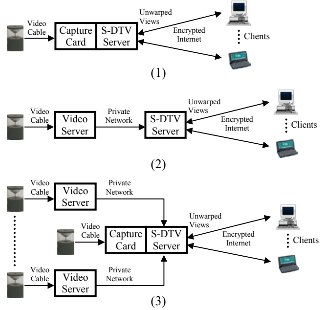
Figure 5. Direct video link, distributed video link, and hybrid configurations of the S-DTV server.
