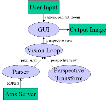
Figure 4. DTV application code flowchart.
