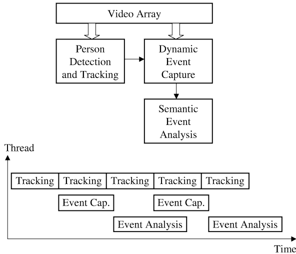
Fig. 8. System processes and multitread synchronization for active event capturing.
