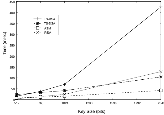
(a) Signature Generation
