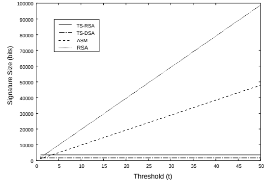
Fig. 10. Signature Size
