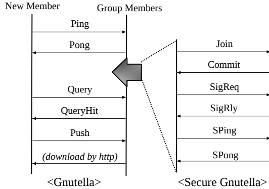
Fig. 6. Secure Gnutella Protocol Flow
