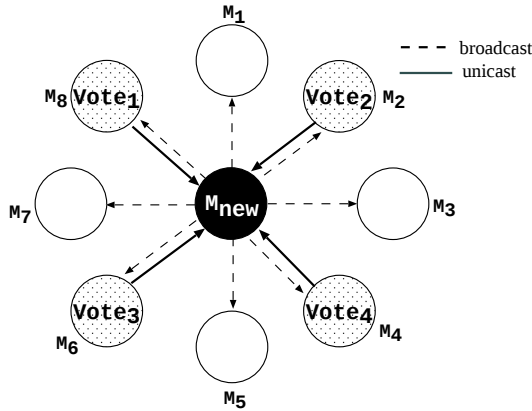
Figure 1: Admission Control
