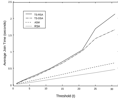
(b) Gnutella
