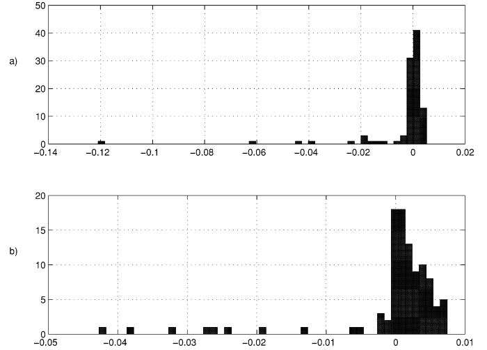
Fig. 2. Histogram of \epsilon_{\text{FOC}}^2 - \epsilon_{\text{OMP}}^2 with SNR = 20 dB, r = 7 , p = 0 . (a) C = 0.8 . (b) C = 1.2 .
