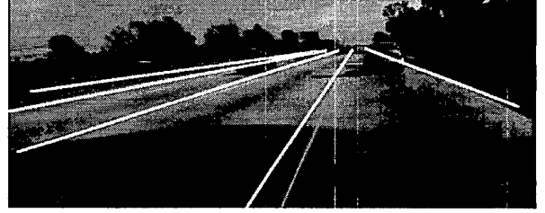
Figure 9 Results during a lane change. (Frame 258 of the test sequence)
