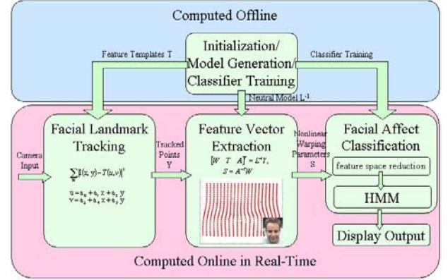
Figure 3: Real-time Affect Analysis System (RAAS) Flow Chart
