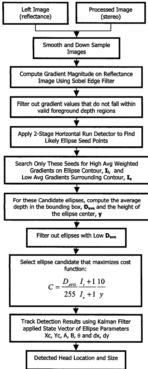
Figure 1 – Head Detection Algorithm Flowchart
