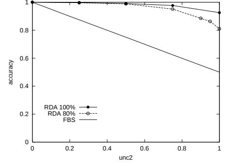
Figure 13: acc = f(unc_2) , L = 5
