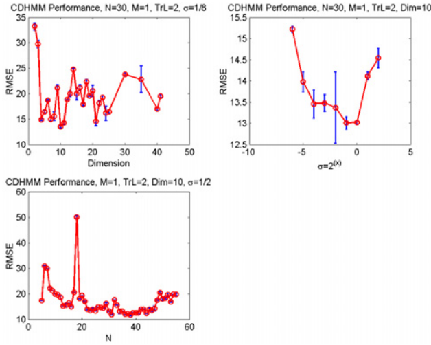
Figure 6. CDHMM performance in terms of the root MSE (RMSE) of the estimates to the ground truth. Top-left: Versus effective dimensions Dim with numbers of states N=30 , Gaussian mixtures M=1 , transition length TrL=2 , initial covariance of the Gaussian likelihoods \sigma=1/8 . The minimum RMSE occurs when Dim=10 . Top-right: Versus \sigma with N=30 , M=1 , TrL=2 , and Dim=10 . Minimum RMSE
