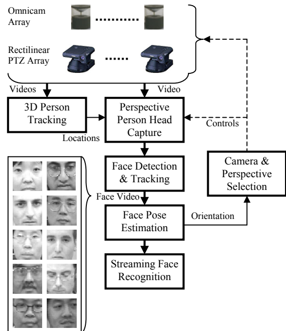
Figure 1. An integrated system for person tracking and identification. It uses video arrays for multiple person tracking and captures high resolution video using the most appropriate camera. Captured video is analyzed for person identification or verification.
