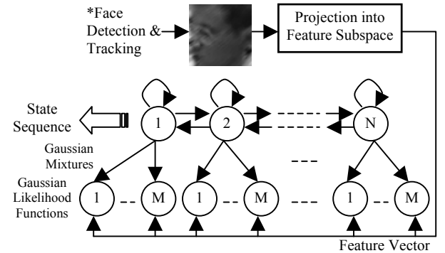
Figure 4. Modified face orientation estimation by continuous density HMM. Face video is projected into feature subspace and generates M Gaussian likelihood values.
