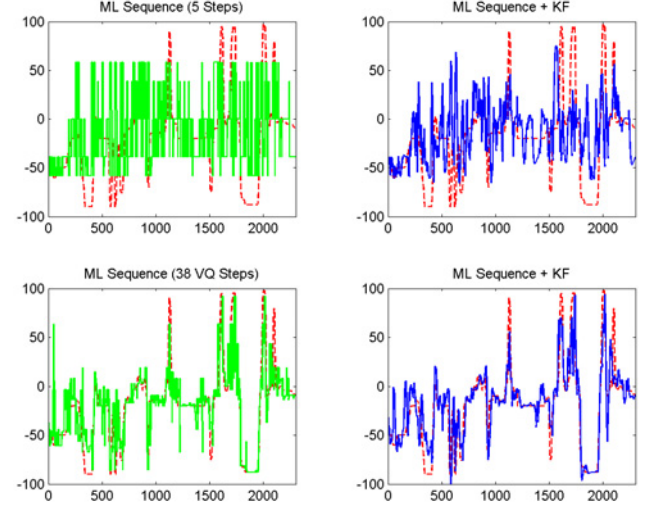
Figure 7. Face orientation estimation performance of the Kalman filter based scheme in Figure 3. The left column shows the ML sequence of 5 quantization steps as described in Section 3 and of the 38 observation likelihood functions borrowed from the CDHMM training. The right column shows the Kalman filtered ML sequences. The solid line is the estimated face orientation, and the dotted line is the ground truth value.
