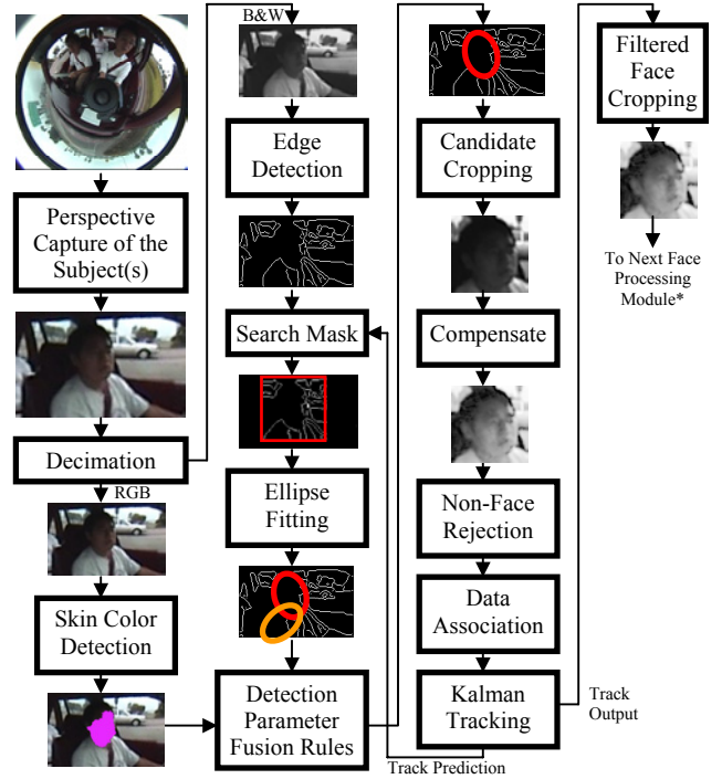
Figure 2. The computational flow chart for the integrated "closed-loop" head/face detection and tracking modules.
