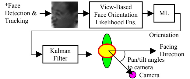
Figure 3. The first scheme of face orientation estimation.
