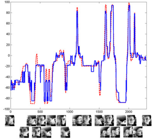
Figure 8. Face orientation estimation of the CDHMM scheme in Figure 4. The horizontal axis is the frame number. The solid line is the estimated face orientation, and the dotted line is the ground truth value. The CDHMM configurations are N=38 , M=1 , Dim=10 , TrL=2 , and \sigma=1/2 .
