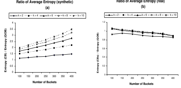
Figure 9: Change in Entropy a)Synthetic b) Real data
