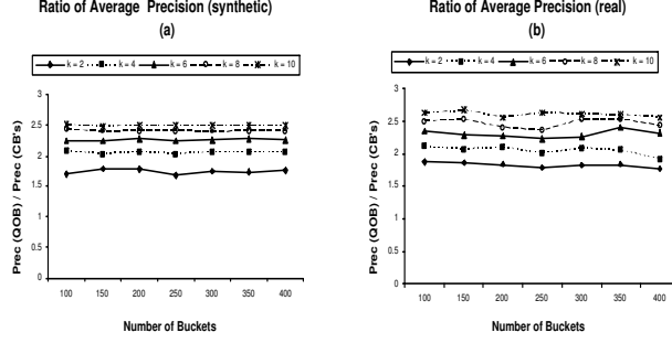
Figure 7: Decrease in Precision a)Synthetic b) Real data
