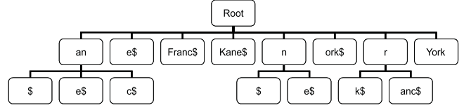
Figure 7: Suffix Tree : Example
