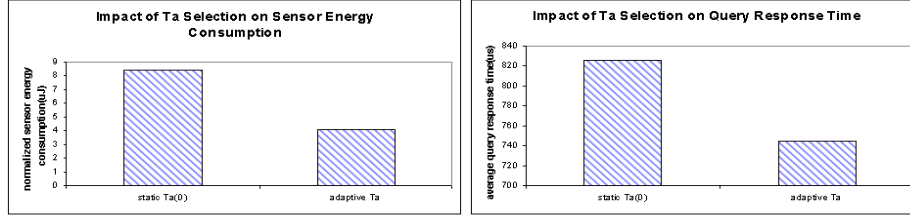
Figure 6: Impact of T_a adaptation on system performance
