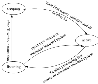
Figure 4: The Active-Listening-Sleeping model
