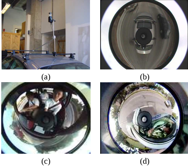
Figure 1: (a) Vehicle Test Platform with omni camera mounted two feet above the roof using a specially designed fixture. (b) Omni-directional image acquired the camera. (c) and (d) Image from omni-camera mounted inside the car and on side of the car respectively.
