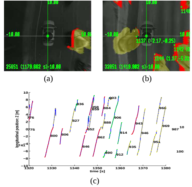
Figure 5: Surround analysis in different situations with the top mounted camera: (a) City road (b) Freeway (c) Plot of the longitudinal position of vehicle tracks against time. The tracks are color coded as red, yellow and green according to increasing lateral distance from the ego-vehicle.
