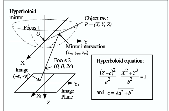
Figure 3: Omni-directional camera geometry.
