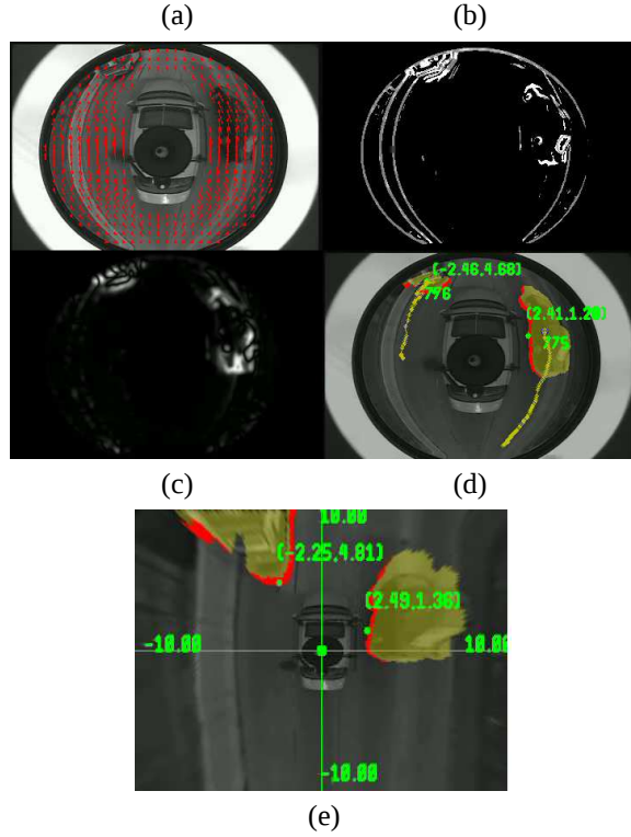
Figure 4: (a) Image from a sequence using omni camera mounted on a moving car with estimated parametric motion of ground plane. (b) Classification of points into inliers (gray), outliers (white), and unused (black). (c) Normalized difference between motion-compensated images. (d) Detection and tracking of moving vehicles marked with track id and the coordinates in road plane. (e) Surround view generated by dewarping omni image.
