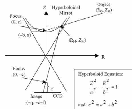
Figure 2 – Model of omnidirectional mirror in relation to the CCD
