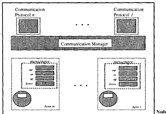
Figure 3. CRCF model: Each base level actor has a meta level actor, called messenger and there is one meta level entity called communication manager in every node of the distributed
