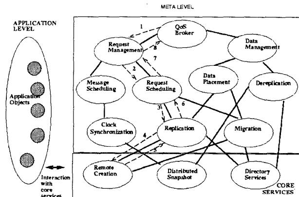
Figure 2. The QoS Broker
