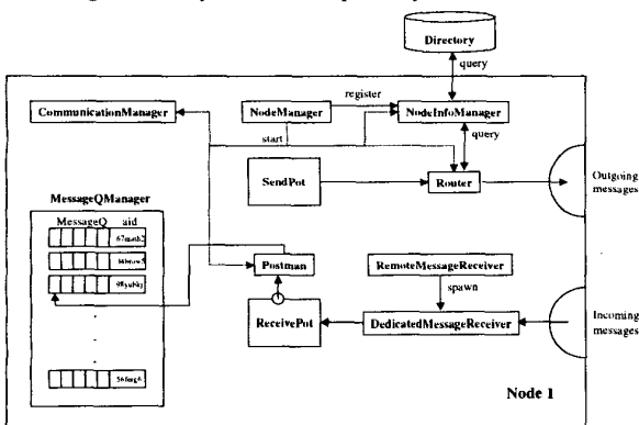
Figure 4. Schematic of the software design for the CompOSEIQ runtime environment.
