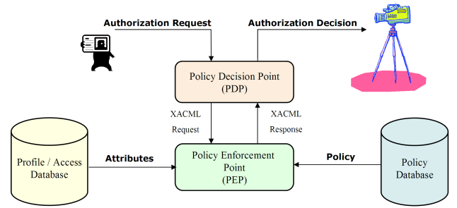
Figure 5: XACML-based Policy Framework.
