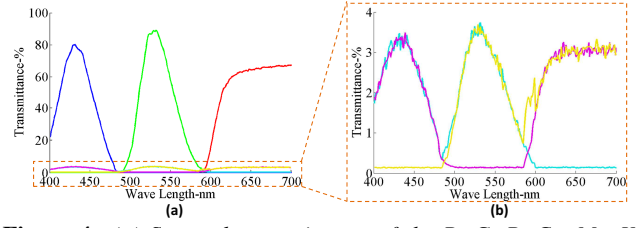
Figure 4: (a) Spectral transmittance of the R, G, B, C_h, M_h, Y_h channels. (b) Zoomed-in view of the spectral transmittance of the C_h, M_h , and Y_h channels. The zoomed-in view shows that the RGB channels extracted from C_h, M_h , and Y_h are similar to the LDR RGB channels but are considerably less sensitive to light.
