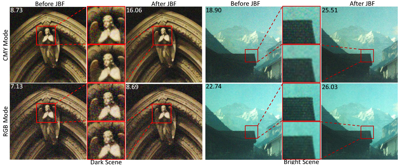
Figure 11: Scenes captured with CMY (top) and RGB (bottom) modes of our camera is shown before (left) and after (right) applying the JBF for a dark and a bright scene. The SNR are embedded on the top left of each image. For the dark scene, the CMY mode provides superior SNR, particularly after applying the JBF. For the bright scene, the RGB mode provides superior SNR. The JBF reduces the noise but degrades the overall perceptual quality of the image because of the reduced sharpness of the edges.
