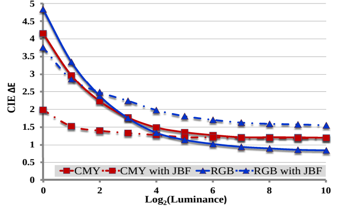
Figure 12: \Delta E difference from ground truth for RGB and CMY modes before and after the JBF. Longer exposure time is used for lower luminance levels such that the amount of light that reaches the sensor remains constant. The longest exposure is 2 seconds and the shortest is 1 millisecond. We used ISO 400. The graph demonstrates that for low luminance levels CMY capture mode is superior particularly after applying the JBF. On the other hand, for high luminance levels RGB capture mode without JBF results in superior fidelity while the JBF degrades the quality of the image.
