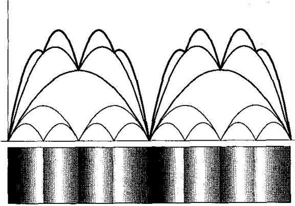
Figure 4. Binary subdivision of interval
