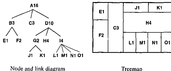
Figure 1. Tree representations
