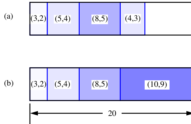
Figure 12.12: An example showing that our first approach to defining a knapsack subproblem does not work. The set S consists of five items denoted by the the ( weight, benefit ) pairs (3, 2) , (5, 4) , (8, 5) , (4, 3) , and (10, 9) . The maximum total weight is W = 20 : (a) best solution with the first four items; (b) best solution with the first five items. We shade each item in proportion to its benefit.
