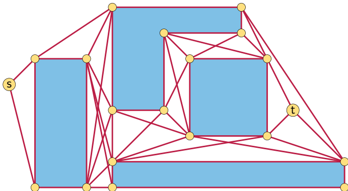
“Visibility graph”
