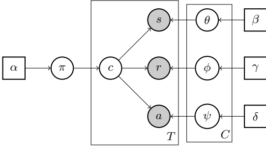
Figure 2: Graphical model for the MPMM.
