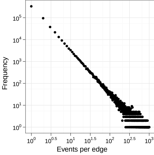
Figure 1: Number of edges for which we observe a given number of events in a data set of international dyadic events [15].
