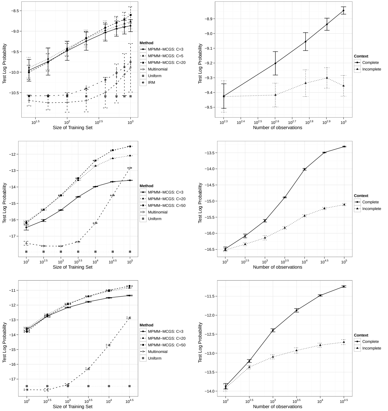
Figure 6: The left-hand plots show the predictive accuracy (measured by test log-likelihood) of different models on real-world data sets. The right panel compares the performance of MPMM with fully observed event data versus partially observed data. Top: Red Deer data set. Center: Email data. Bottom: International dyadic events.
