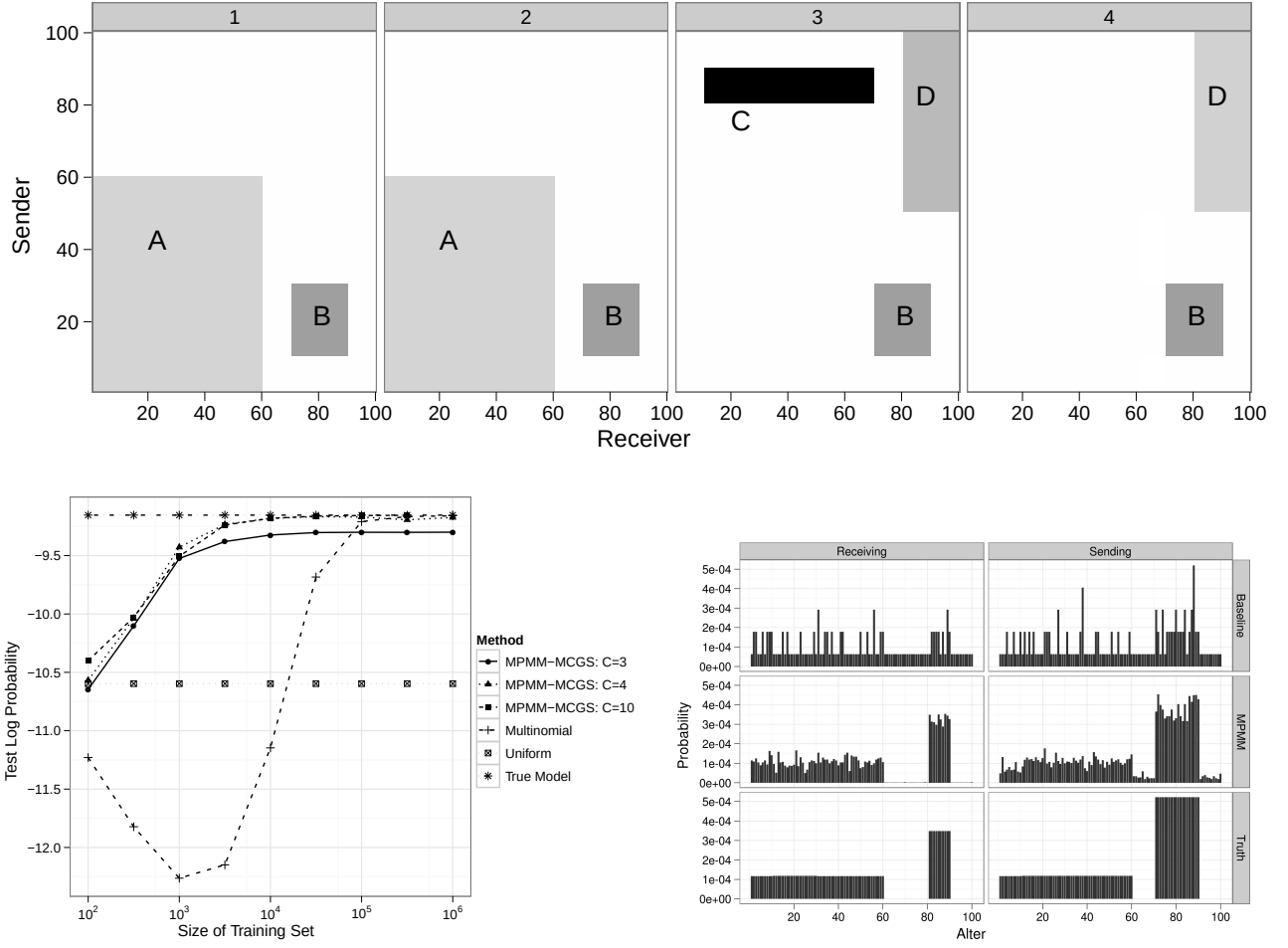
Figure 5: Top: Probability of an event for a synthetic data set with four latent classes labeled A, B, C, and D. Each panel represents an action type. Left: Comparison of test log-likelihood for the synthetic data set using the CGS algorithm with different numbers of latent classes C versus the baseline. See 6 for a discussion. Right: Comparison of predictive distributions between models and truth for actor 30 on a training set of 10000 events with the hyperparameters used in the experiment at left. The MPMM approximation provides a better fit over the typical recipients.
