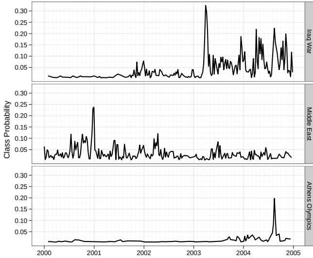
Figure 4: Proportion of assignments per week for latent classes from a data set of international political events [15], with typical senders, receivers, and action types shown in Table 1.
