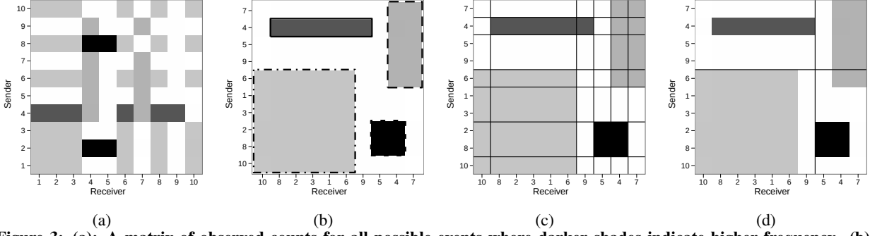
Figure 3: (a): A matrix of observed counts for all possible events where darker shades indicate higher frequency. (b): MPMM models the data via a low-dimensional representation indicating groups of events. This structure is apparent after reordering the rows and columns. Stochastic blockmodels can model such data either by having (c) many small homogeneous blocks or (d) with a few inhomogeneous blocks; the latter misses some of the structure.
