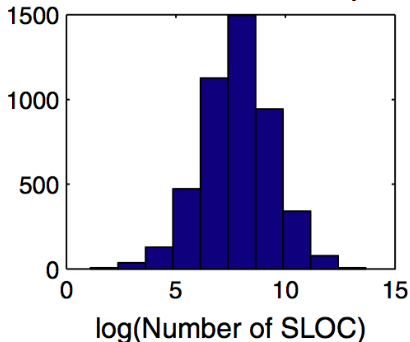
SLOC Distribution over Projects
