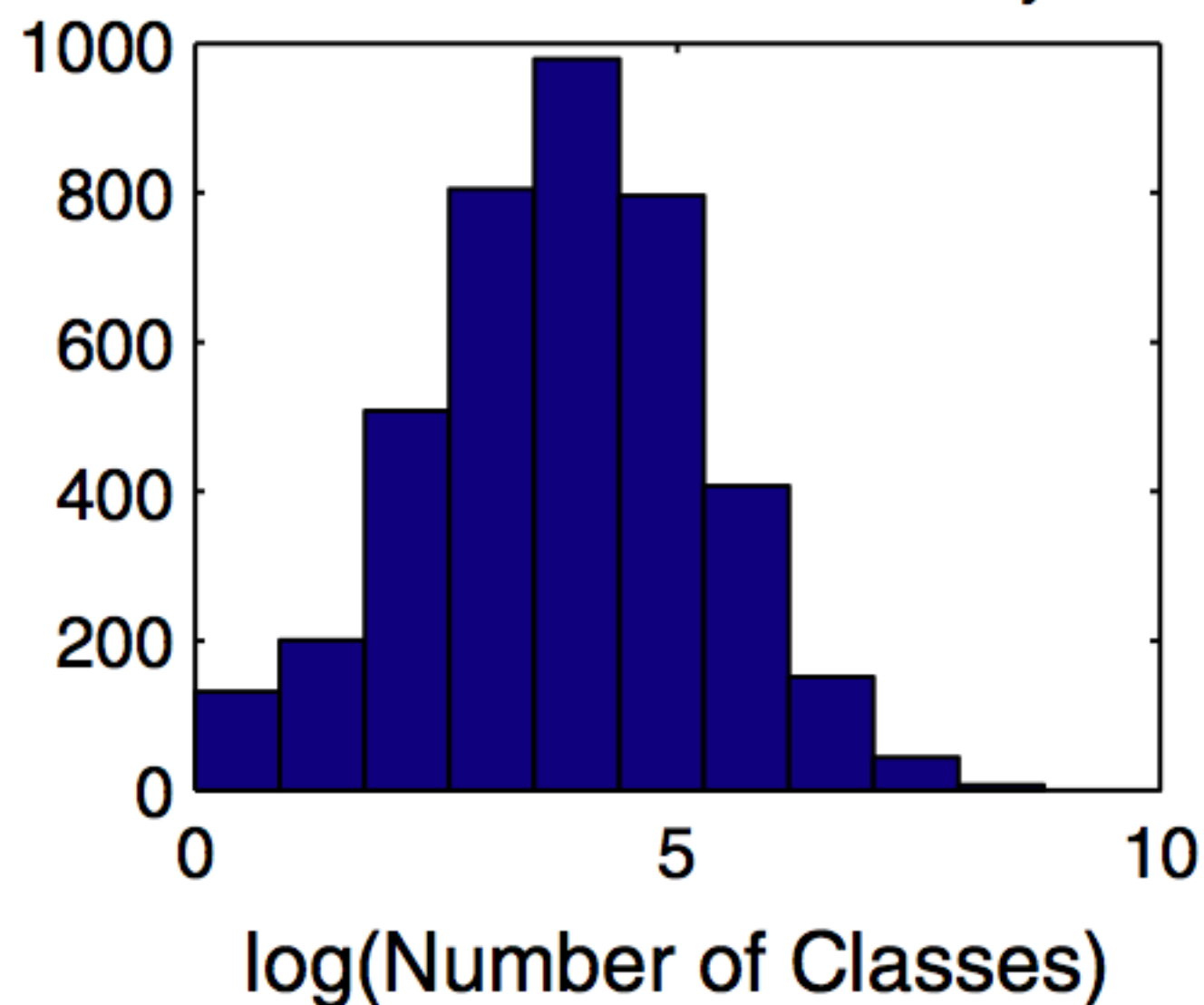
Class Distribution over Projects
