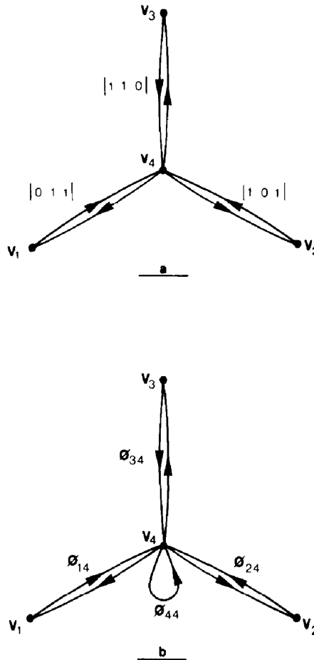
Fig. 4. (a) A symmetric network of constraints. (b) The network of constraints Y' equivalent to (a) computed by algorithm C in one iteration, with order of elimination (4, 1, 2, 3).
