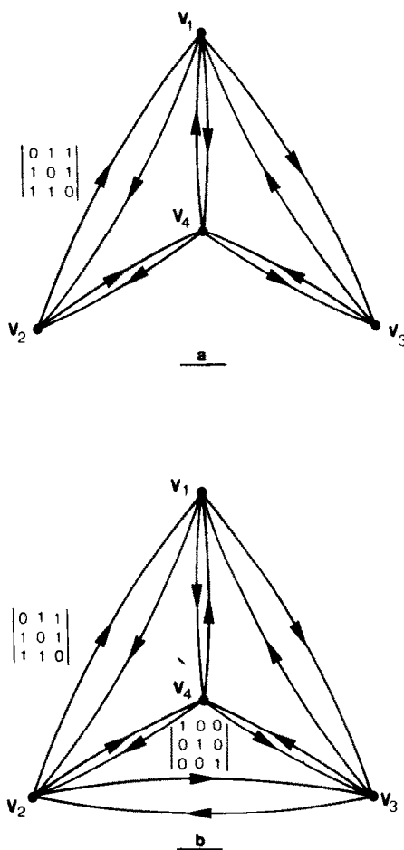
Fig. 5. (a) A series-parallel network with respect to all pairs of vertices except V_2V_3 .
