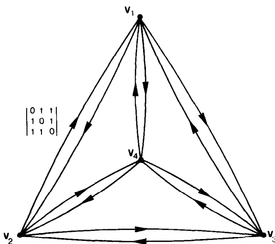
Fig. 3. In this network, the relation \begin{vmatrix} 0 & 1 & 1 \\ 1 & 0 & 1 \\ 1 & 1 & 0 \end{vmatrix} is associated to every arc. This network represents the impossible problem of coloring a four-vertex complete graph with three colors. This network is symmetric and closed but not minimal.
