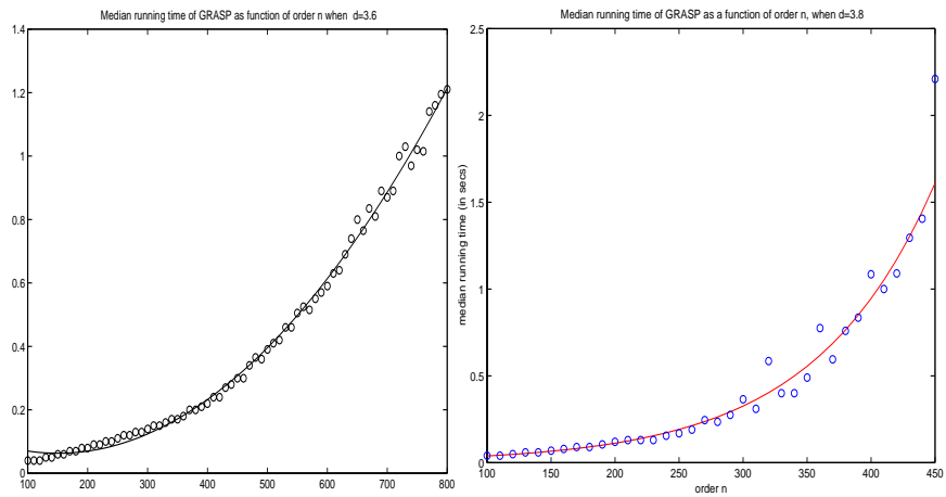
Figure 2. GRASP – median running time for density 3.6 (left) and density 3.8 (right) as a function of the order of the instances. At density 3.6, the best fit curve is quadratic in the order, while at 3.8, the best fit curve is exponential in the order.
