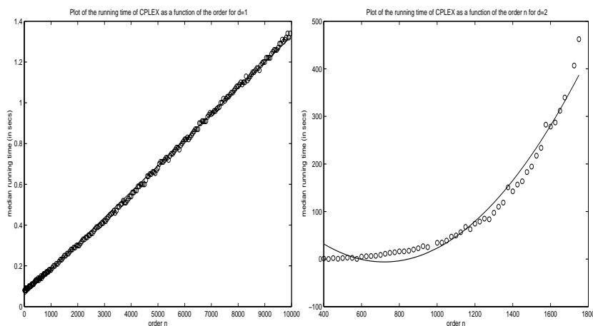
Figure 5. CPLEX – median running time for density 1 (left) and density 2 (right) as a function of the order of the instances.
