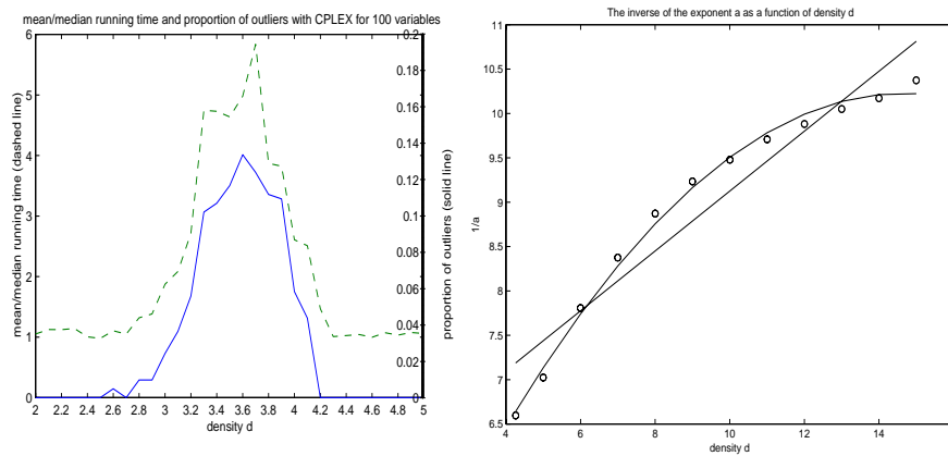
Figure 6. CPLEX – (left) Ratio of mean to median running time and proportion of outliers, and (right) the exponent 1/\alpha of median running time as a function of density.
