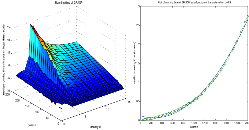
Figure 1. GRASP – (left) 3-D Plot of median running time, and (right) median running time for density 0.9 as a function of the order of the instances. A quadratic function fits these points better (with an r^2 > 0.98 ) than an exponential function.
