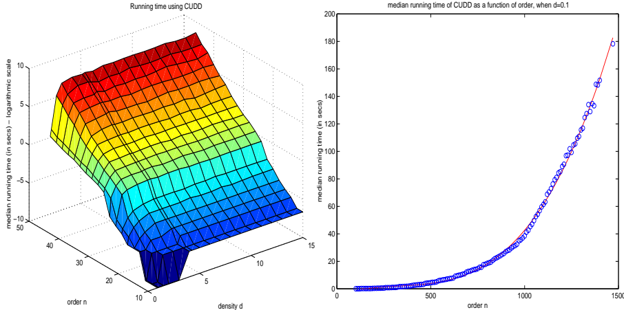
Figure 7. CUDD – (left) 3-D Plot of median running time and (right) median running time for density 0.1
