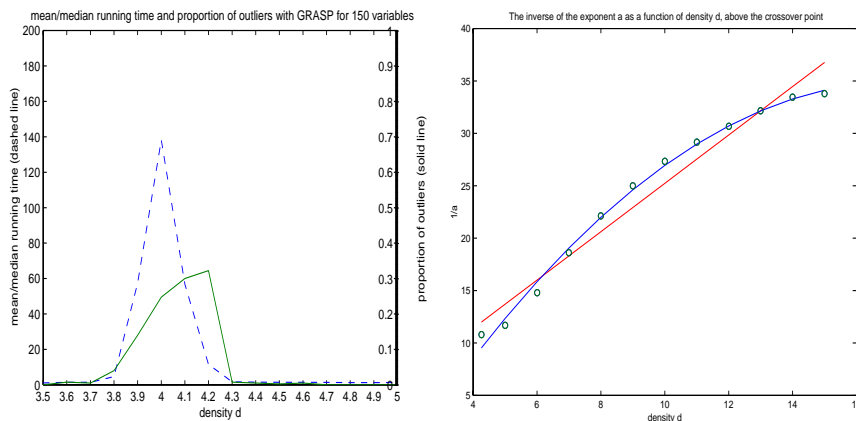
Figure 3. GRASP – (left) Ratio of mean to median running time and the proportion of outliers, and (right) the exponent 1/\alpha of median running time as a function of density.
