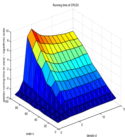
Figure 4. CPLEX – 3-D Plot of median running time
