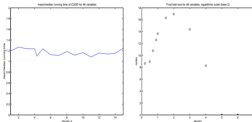
Figure 8. CUDD – (left) Ratio of mean to median running time and (right) median ROBDD size as a function of density
