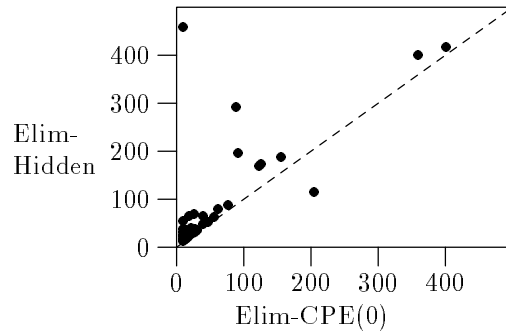
Figure 12: 50 test instances of the insurance network with query parameters \langle 15, 5 \rangle
