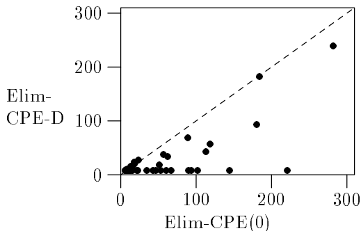
Figure 9: 48 test instances with network parameters \langle 80, 4, 0.75 \rangle and query parameters \langle 0, 10 \rangle
