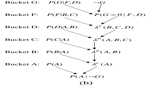
Figure 4: Variable elimination for a hybrid network: (a) Elim-CPE with clause extraction (b) regular Elim-CPE
