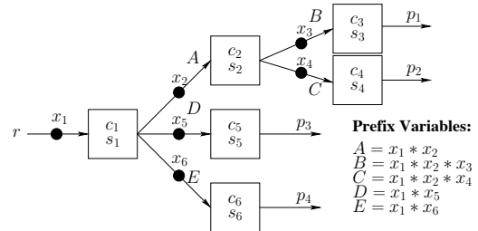
Figure 3: Two levels of operator splits
