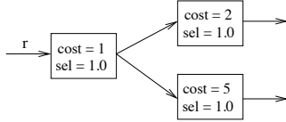
Figure 7: Splits supported by complementary plans
