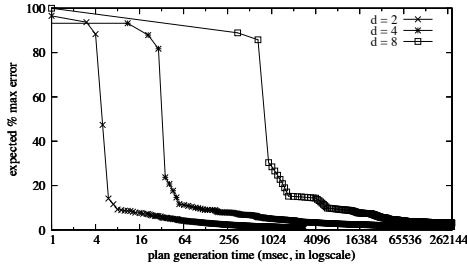
(a) Convergence of exp. \epsilon_{max} for Solver-W
