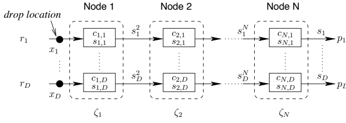
Figure 2: Linear query diagram and notation
