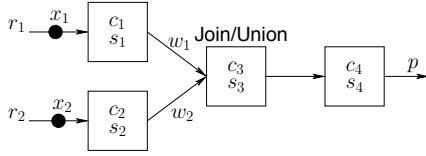
Figure 4: Merging two streams via Join or Union
