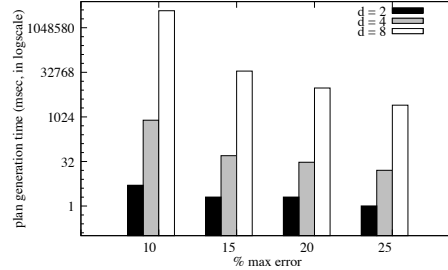
(b) Effect of dimensionality on C-FIT
