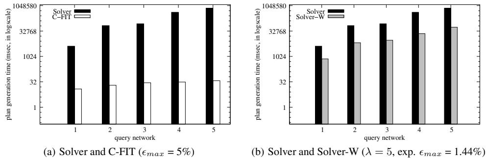
Figure 10: Effect of query load imbalance
