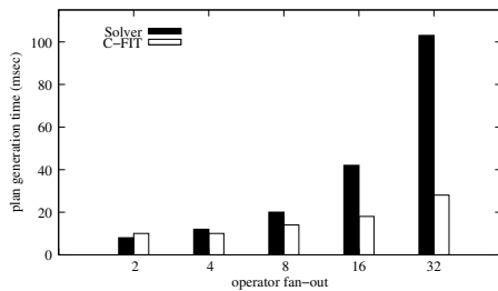
Figure 13: Effect of operator fan-out ( \epsilon_{max} = 1\% )
