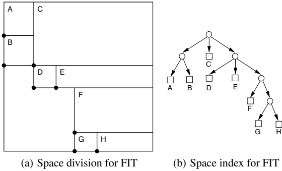
Figure 8: Point-Quadtree-based space division and index
