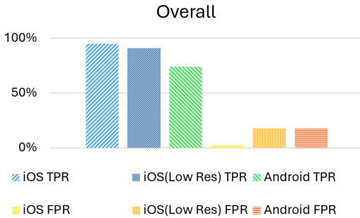
Figure 13: Overall effectiveness of Scoop's prototype.
