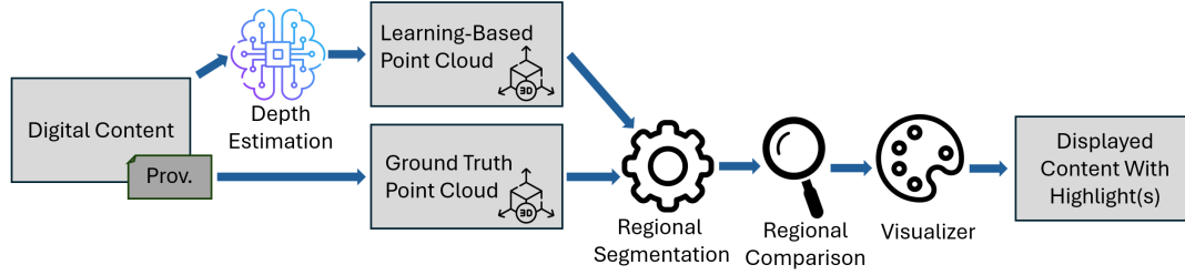
Figure 7: Scoop viewer's workflow.
