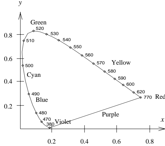
Figure 1: CIE chromaticity diagram, wavelengths (in nanometres) and positions of saturated colours specified on the boundary of the horseshoe
